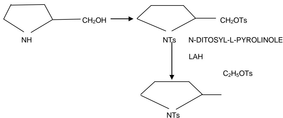
Fig 1: Reaction Mechanism of M 2 Crystal
